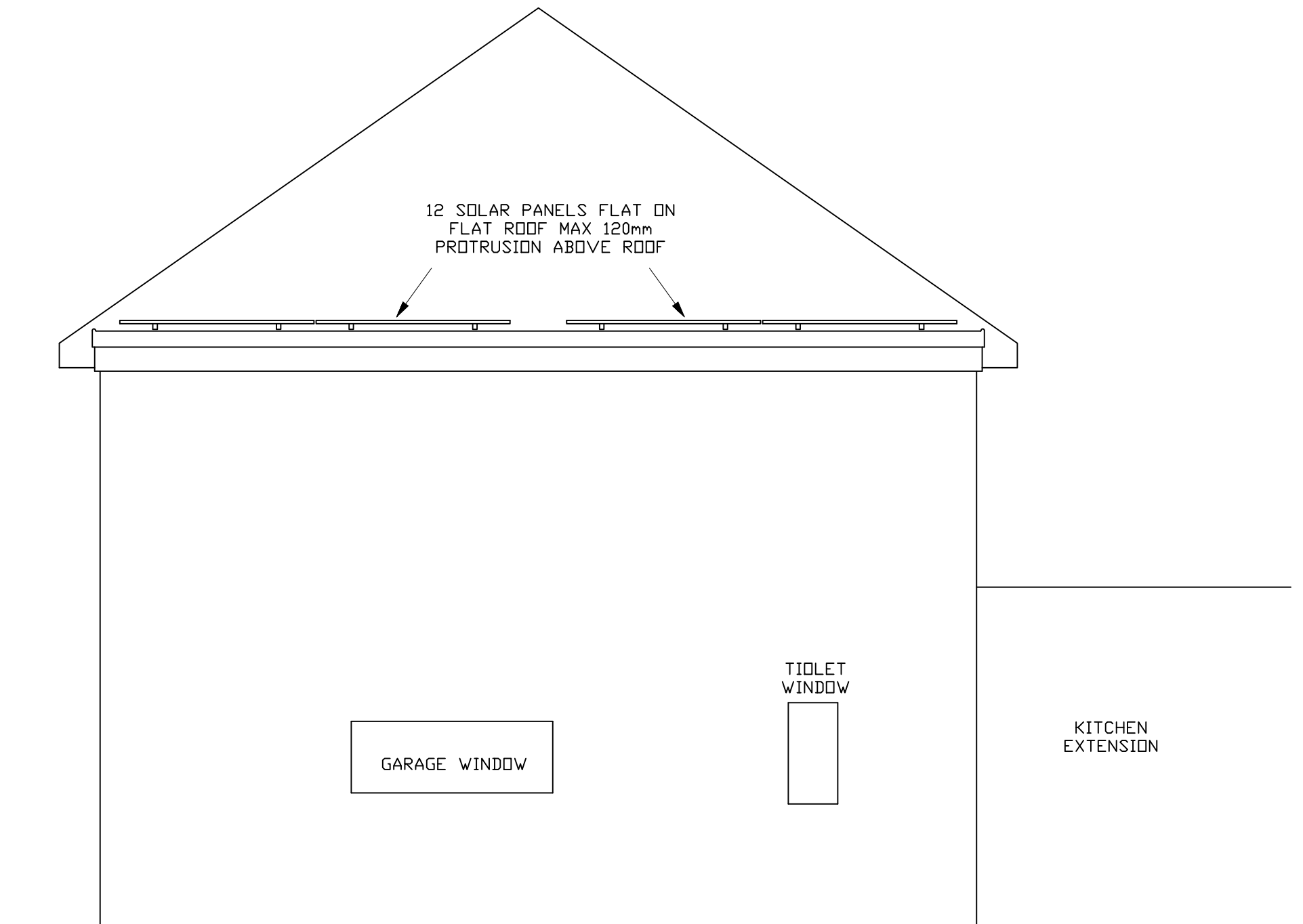
SIDE ELEVATION
